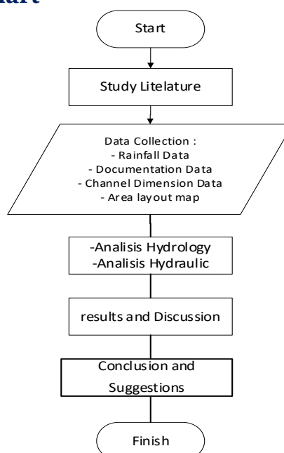
Figure 1. Research Flowchart
