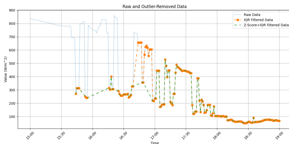
Figure 8. Filtering outliers in radiation data
