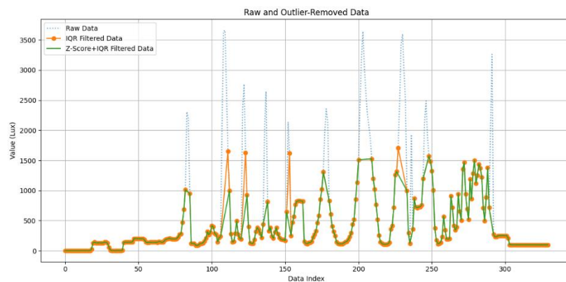
Figure 6. Filtering outliers in test data obtained in the test chamber
