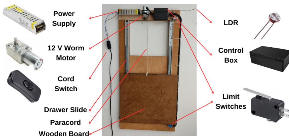
Figure 1. Overview of the Developed Automatic Chicken Coop Door System
