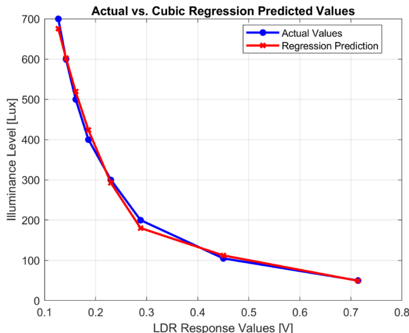
Figure 5. Regression results for LDR to Lux Conversions
