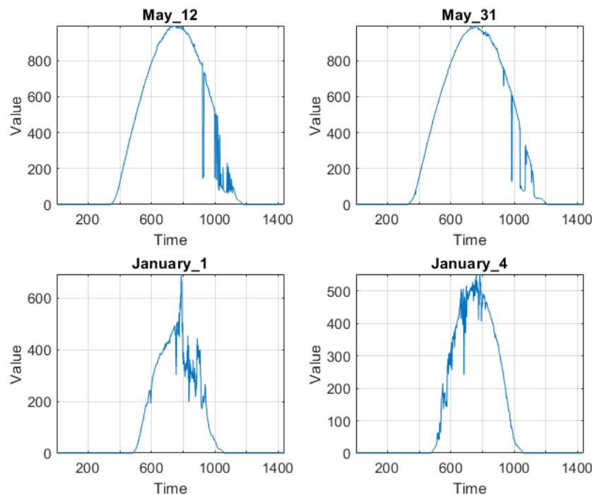
Figure 7. Solar radiation sample values
