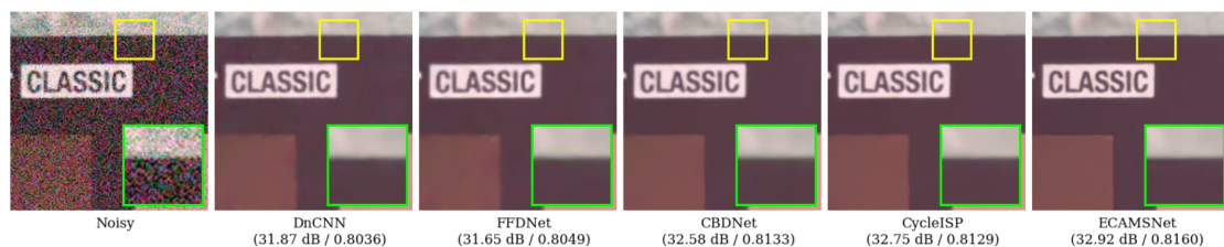
Figure 3. Visual comparison of denoised images for a classic signboard from the SIDD dataset, with zoomed-in regions highlighting text clarity
