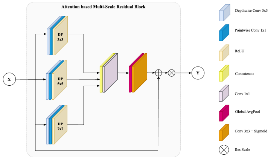
Figure 1. Structure of the AMSRB with parallel 3x3, 5x5, 7x7 convolutions and residual connection
