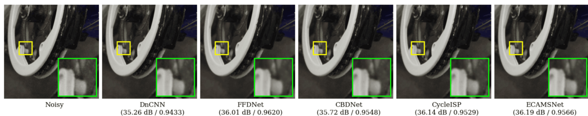
Figure 7. Visual comparison of denoised images for a bicycle wheel from the PolyU dataset, showcasing edge detail.
