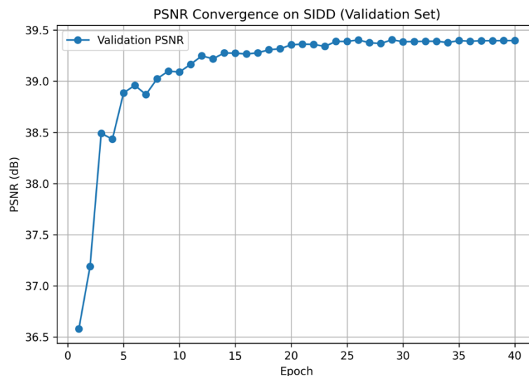
Figure 8. Convergence plot of validation PSNR on the SIDD dataset over 40 epochs, demonstrating the training stability and performance improvement of ECA-MSNet
