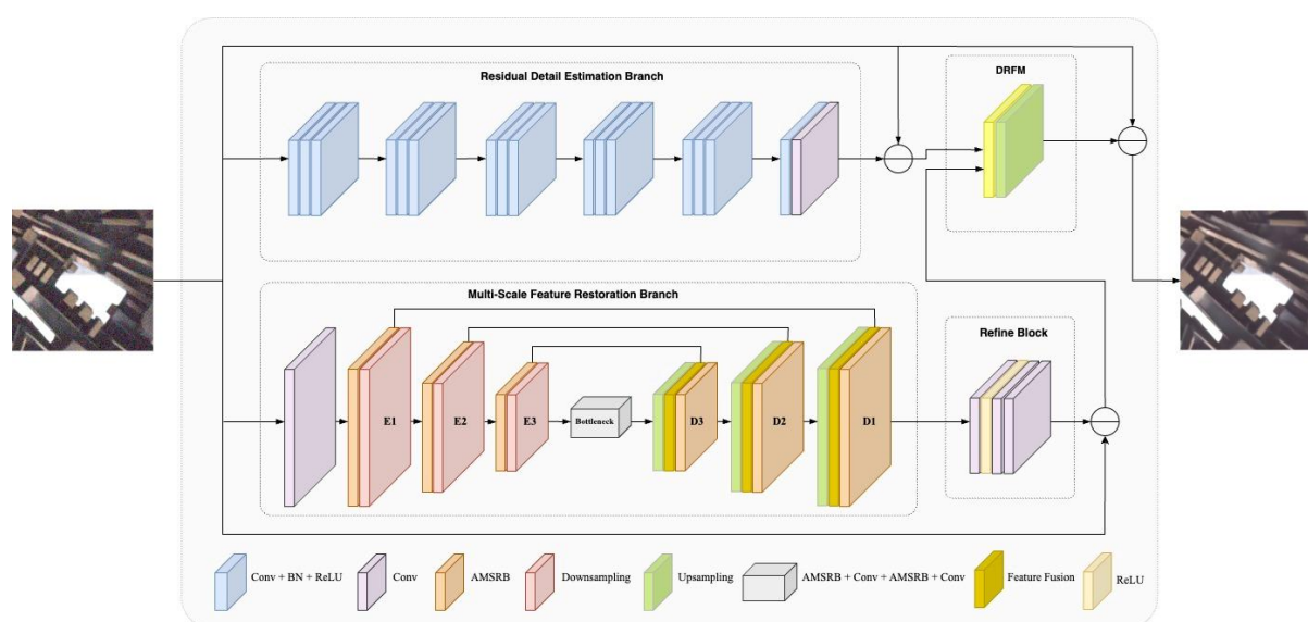
Figure 1. Overview of the ECA-MSNet architecture, illustrating the dual-branch design with a detail estimation branch, a multi-scale feature restoration branch, and a fusion module for image denoising
