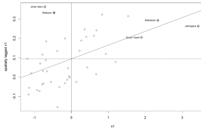
Figure 4. Moran's Scatterplot
