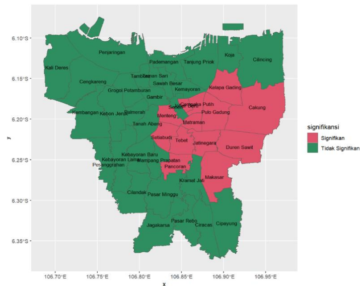
Figure 6. Significance Map
