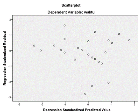
Figure 3. scatter plot results
