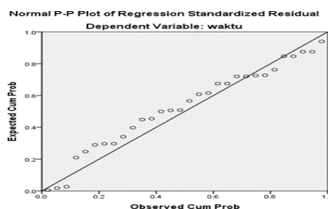
Figure 2. Normal P-Plot of Linear Regression
