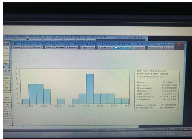
Figure 3. Normality Test
