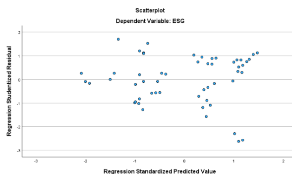
Figure 2. Heteroscedasticity Test
