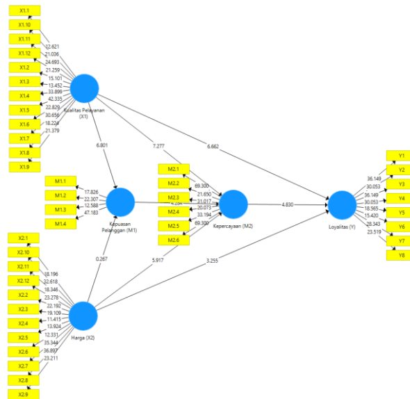
Figure 1. T-Statistics and Bootstrapping Model Source: processed data (2024)
