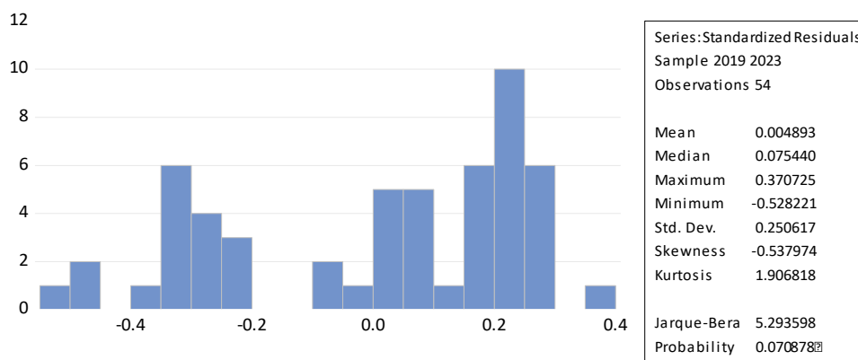
Figure 3. Normality Test
