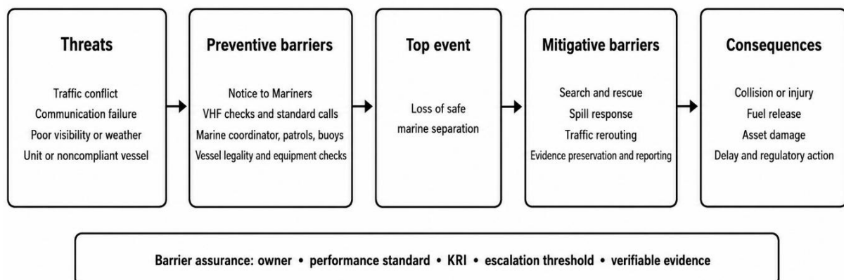
Figure 3. BowTie Barrier Architecture for Loss of Safe Marine Separation (BT-04)
