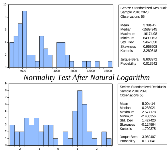
Figure 1 Normality test result
