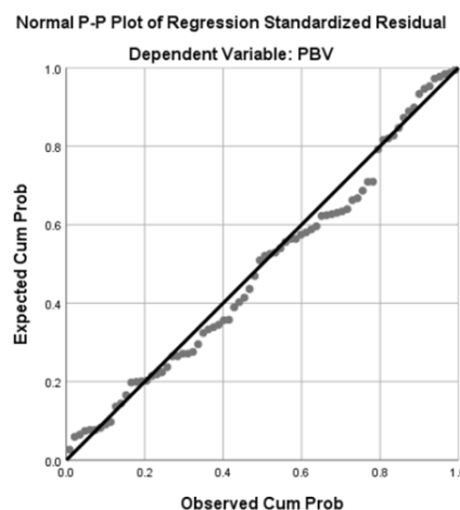
Figure 2. Normality Test Results with P – P Plot
