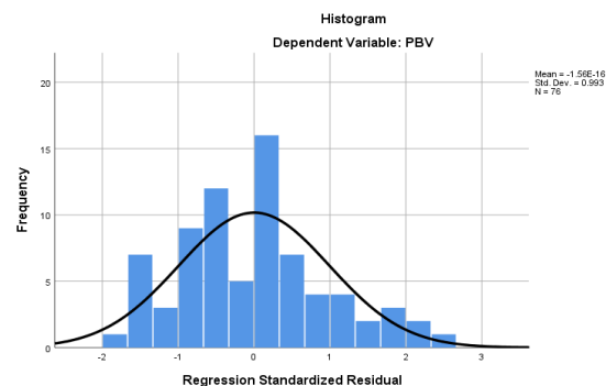
Figure 1. Normality Test Results with Histograms
