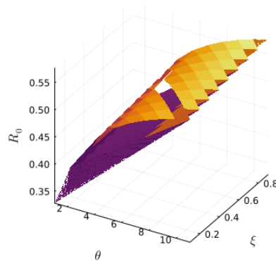
Figure 5. Sensitivity of the basic reproduction number to the parameters \theta and \xi
