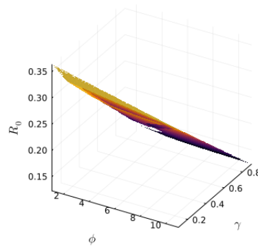
Figure 2. Sensitivity of R_0 to the parameters \phi and \gamma
