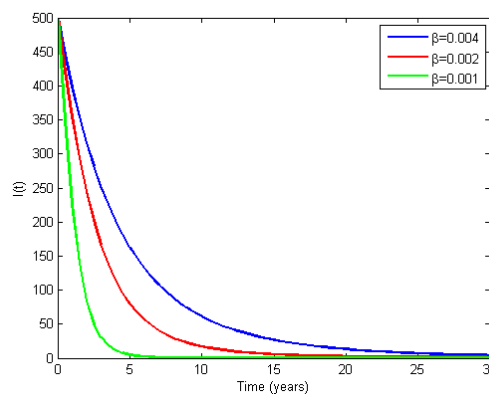
Figure 7. Effect of Contact Rate ( \beta ) of the Infected Population I(t)
