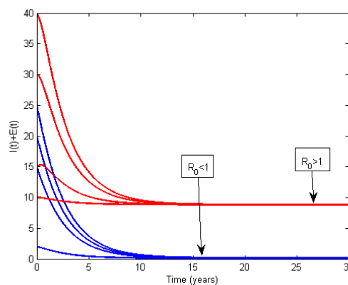
Figure 6. Global asymptotic stability of both endemic and disease-free equilibria of infectious human population
