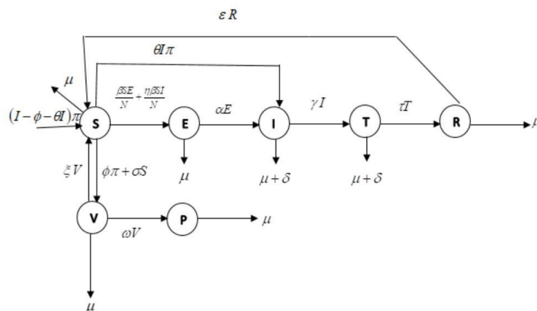
Figure 1. Rubella Disease Model Diagram
