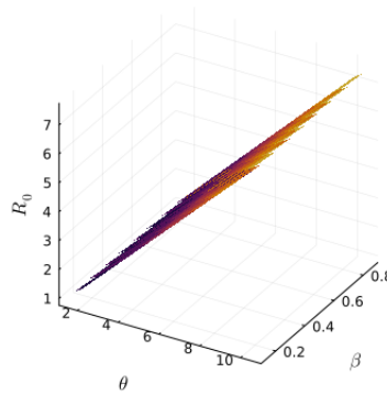
Figure 3. Sensitivity of the basic reproduction number to the parameters \beta and \theta
