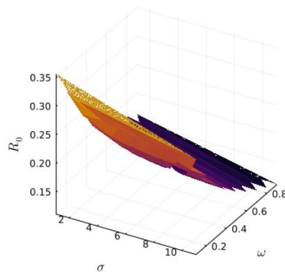
Figure 4. Sensitivity evaluation of R_0 with respect to parameters \sigma and \omega
